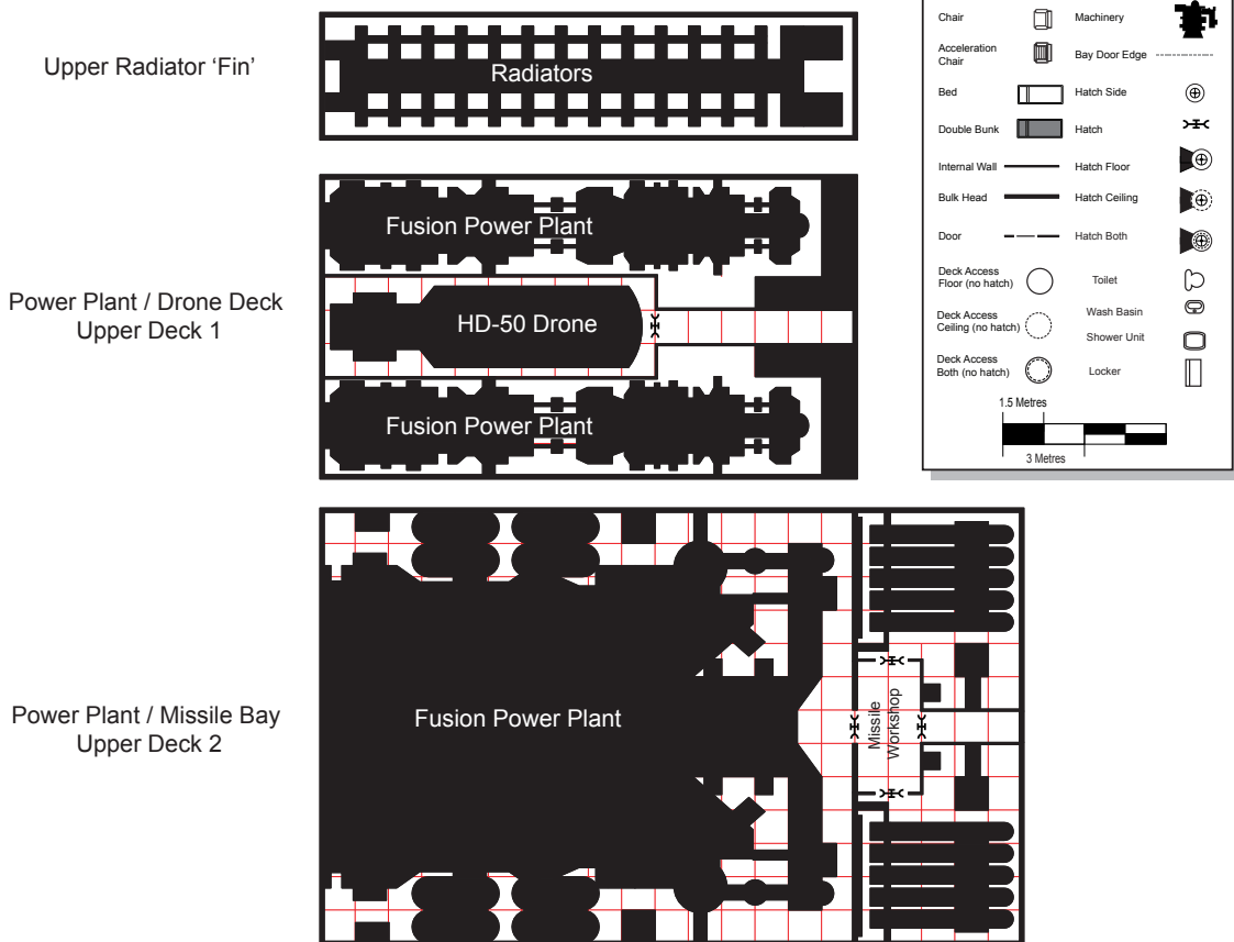
SIM-14 Missile Bay (Upper section)
